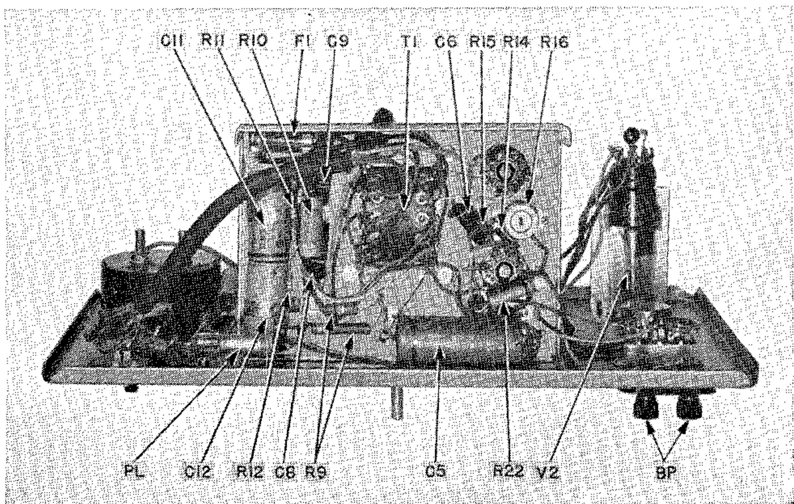
BOTTOM VIEW OF CHASSIS
